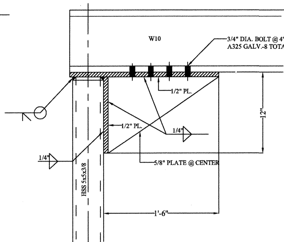
DETAIL 2 NTS
