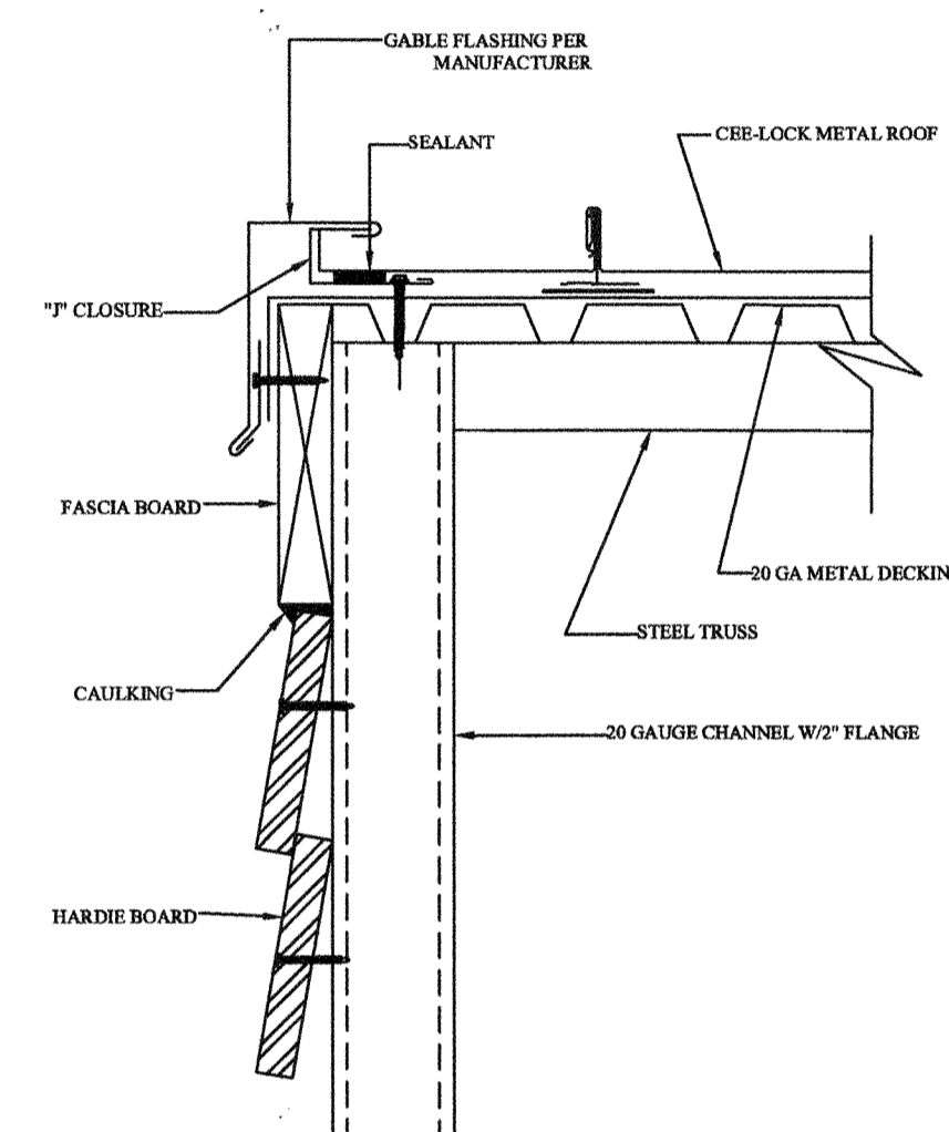
SECTION @ GABLE END NTS
