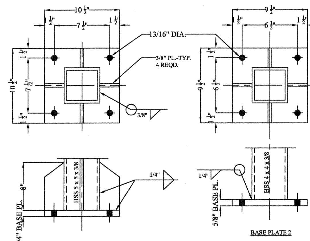
BASE PLATE DETAILS NTS
