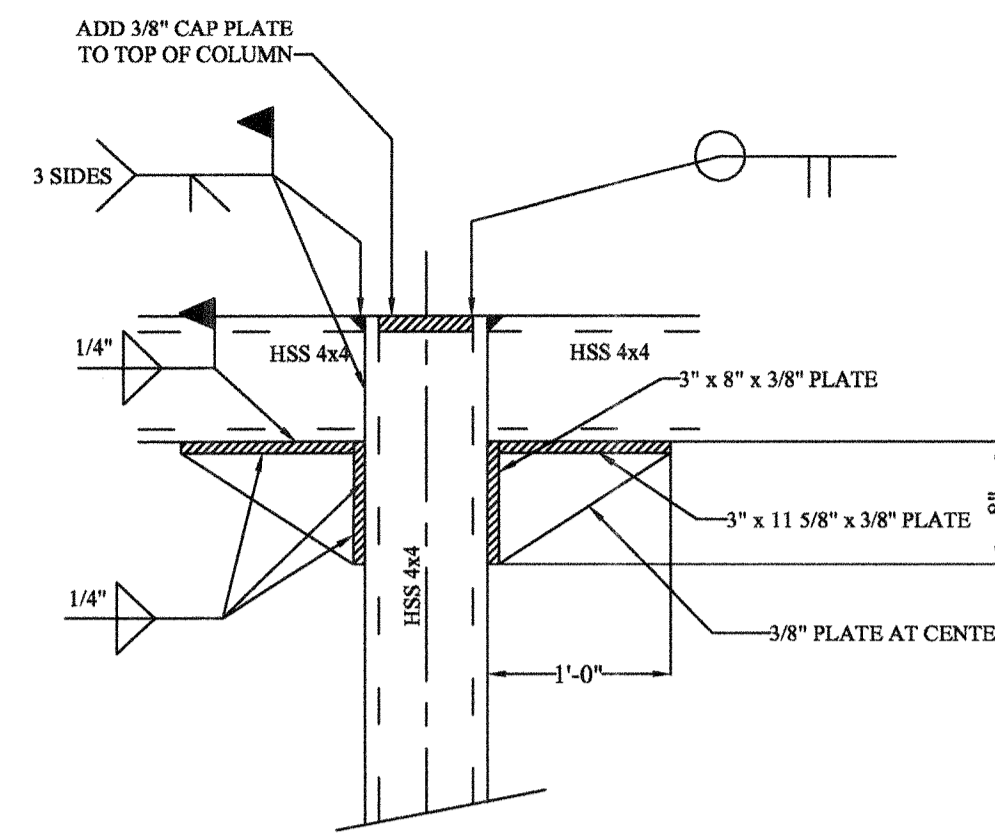
DETAIL 3 NTS
