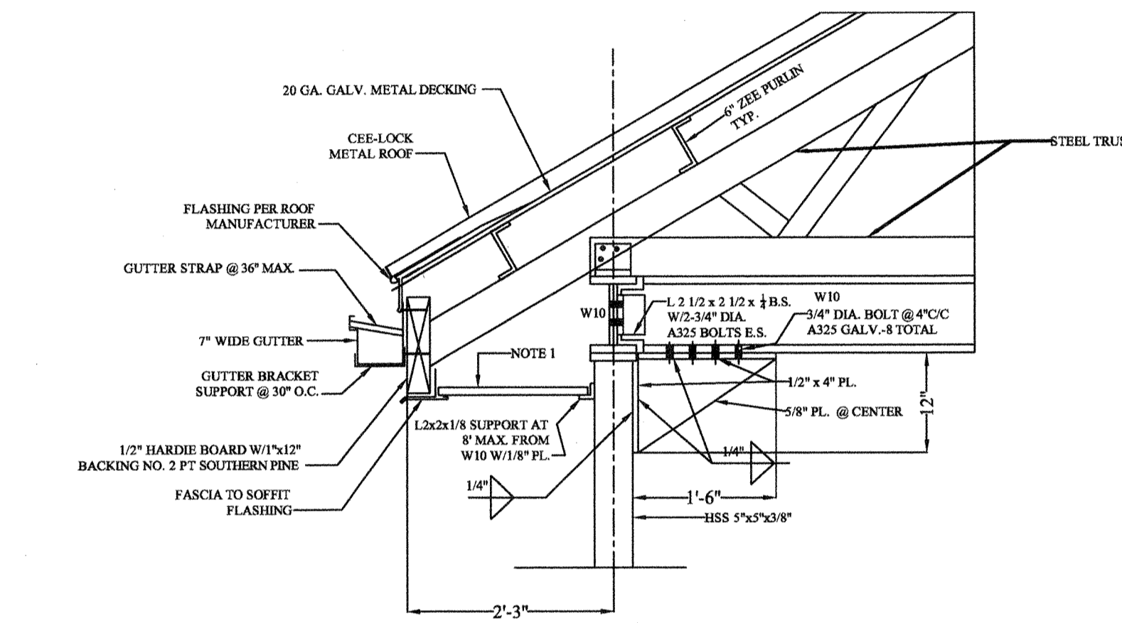
SOFFIT DETAIL NTS
