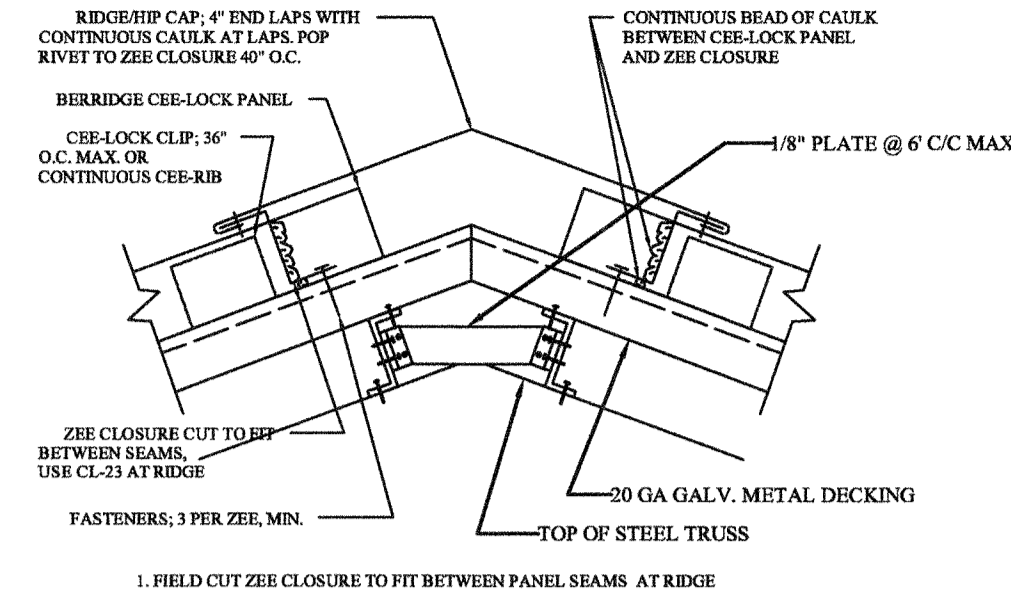
RIDGE DETAIL NTS
