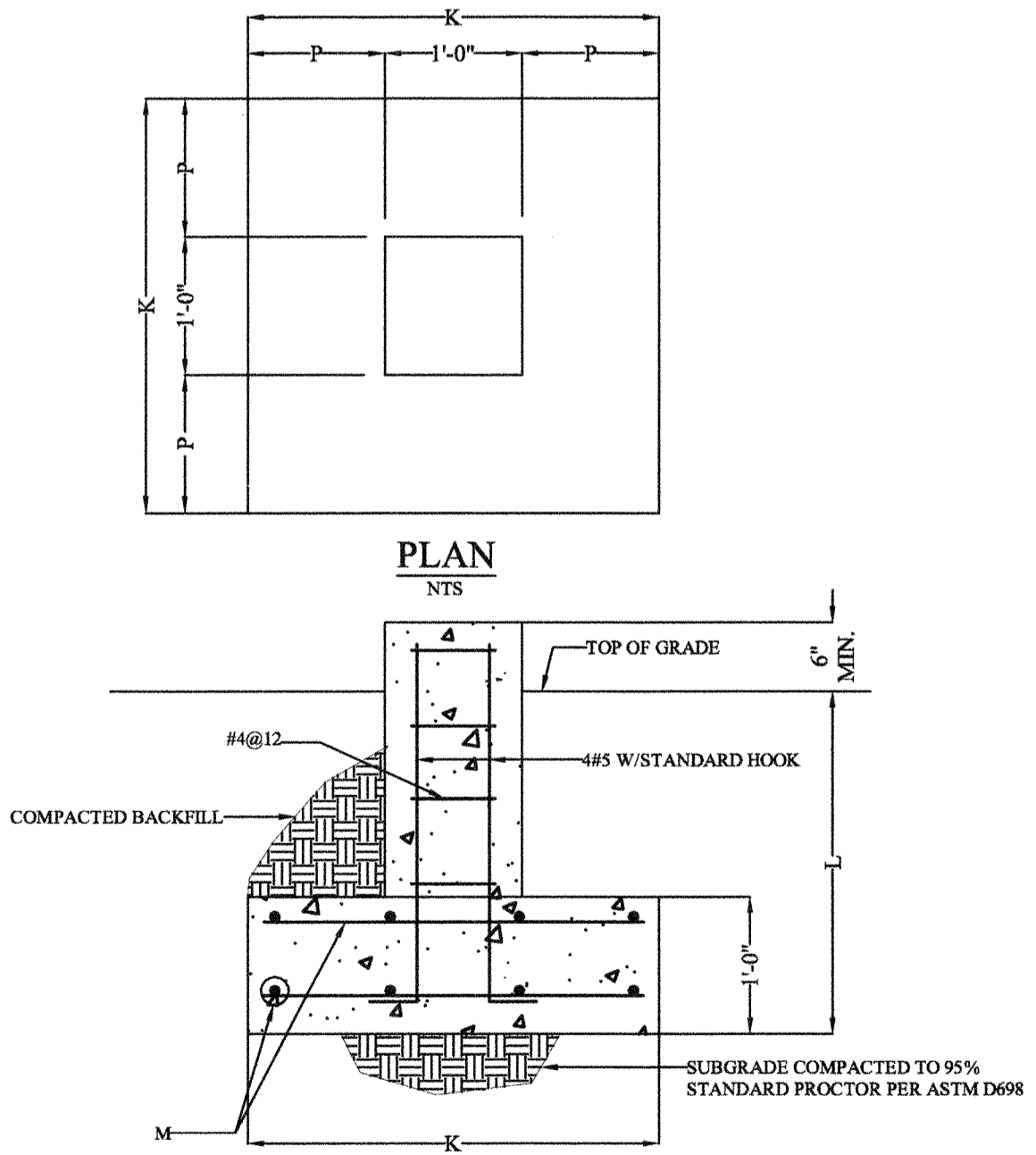
FOOTING DETAIL "A", "B", "C" NTS
