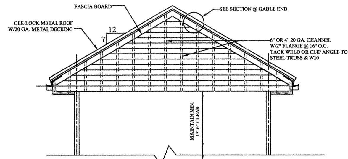
COVERED DRIVE-THRU FRONT/REAR ELEVATION 3/16\"/>
