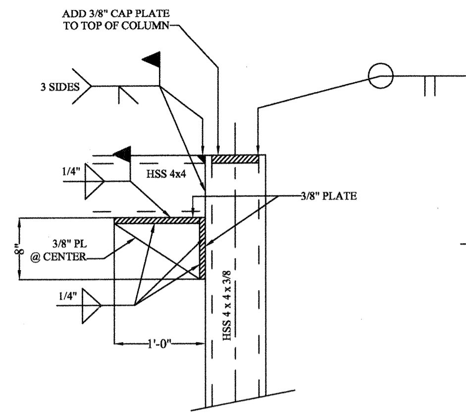
DETAIL 1 NTS
