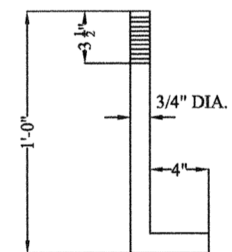
ANCHOR BOLT DETAIL NTS
